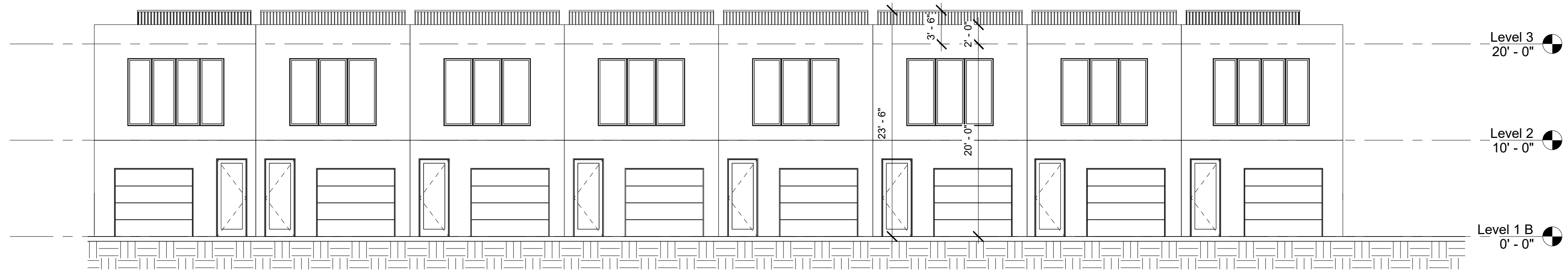
① North 1/8" = 1'-0"
