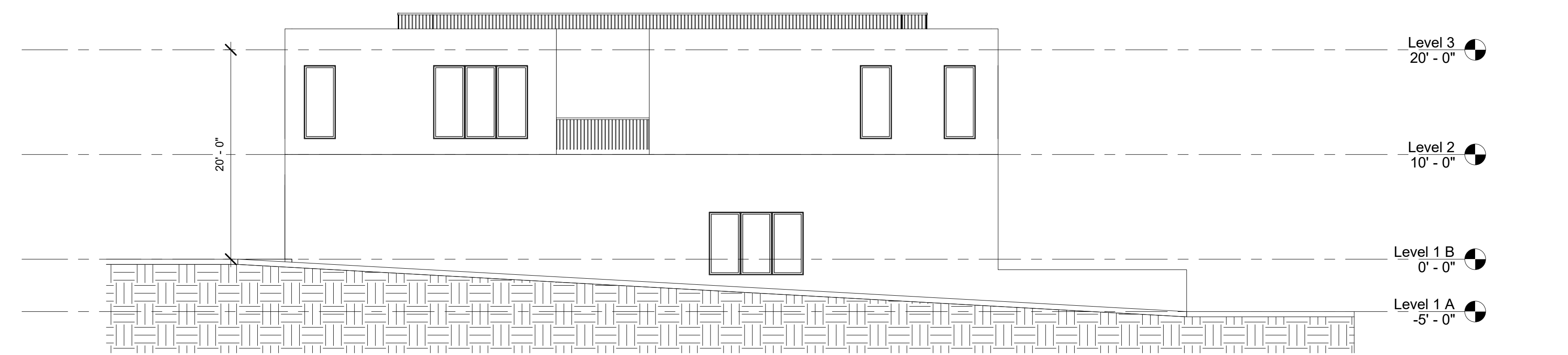
③ West 1/8" = 1'-0"
